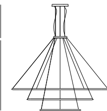
G Ø3000+2000 +1200 mm
